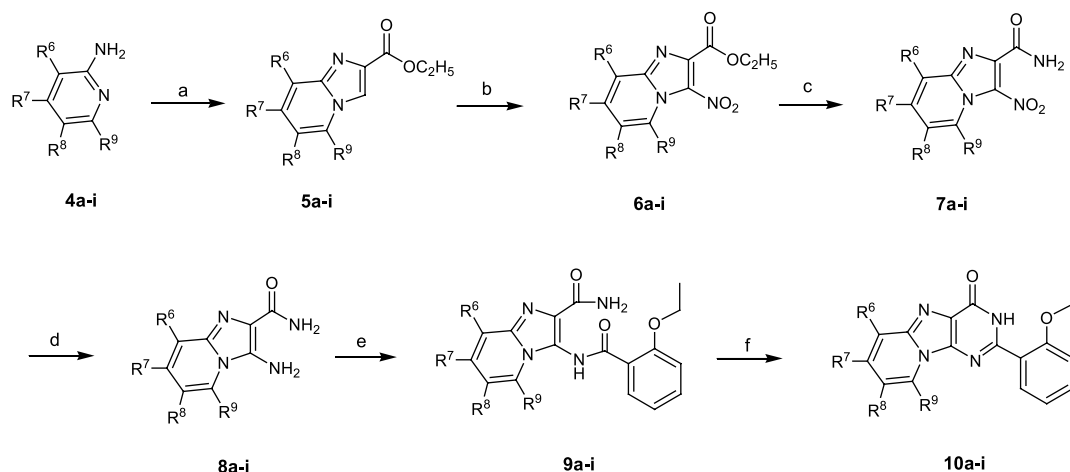
Scheme 1. Reagents and conditions: (a) ethyl bromopyruvate, EtOH, reflux, 6 h; (b) HNO 3 , H 2 SO 4 , −5–0 °C, 2 h; (c) NH 4 OH, H 2 O, THF, rt overnight; (d) H 2 , 10% Pt–C, 50 °C; (e) 2-ethoxybenzoyl chloride, pyridine, DMAP, CH 2 Cl 2 ; (f) KO t -Bu, t -BuOH, reflux.
