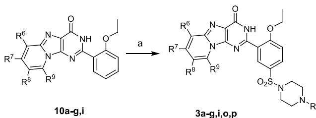
Scheme 3. Reagents and conditions: (a) (i) chlorosulfonic acid, 0–5 °C, 3 h; (ii) N -substituted piperazine, Et 3 N, CHCl 3 , rt, overnight.
