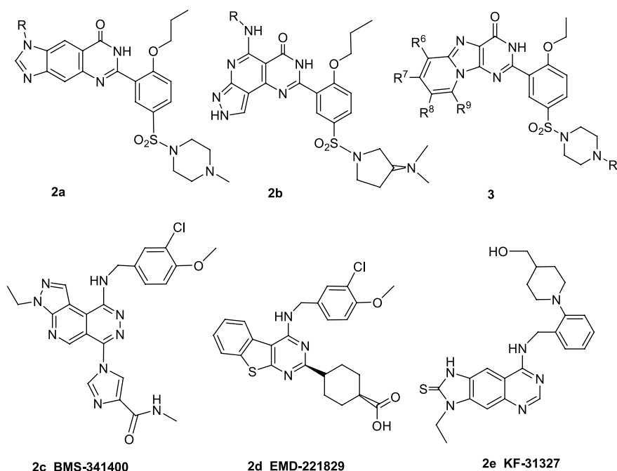
Figure 2. PDE5 inhibitors under development with ‘stretched-out’ purine and other tricyclic skeletons.
