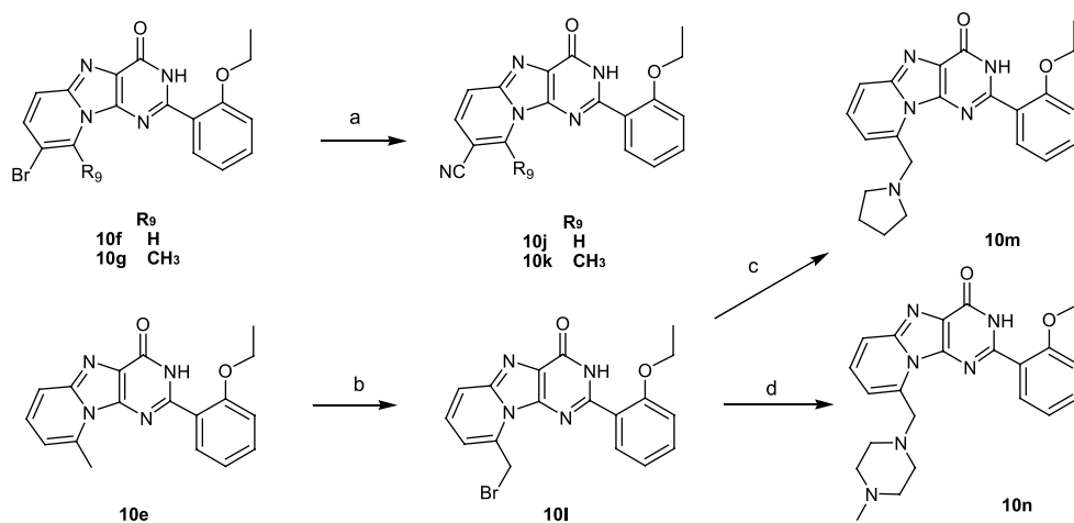
Scheme 2. Reagents and conditions: (a) NaCN, CuI, Pd(PPh 3 ) 4 , DMF, reflux, 24 h; (b) NBS, CCl 4 , hν , 2 h; (c) pyrrolidine, K 2 CO 3 , acetone, rt, 20 h; (d) N -methylpiperazine, K 2 CO 3 , acetone, rt, 20 h.
