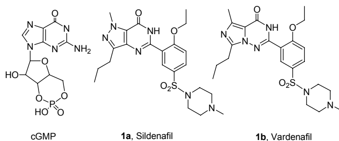
Figure 1. cGMP and PDE5 inhibitors with purine-isosteric heterocyclic systems.
